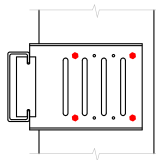
(4) #10 Screw Pattern Shown in a DRC6 Clip
