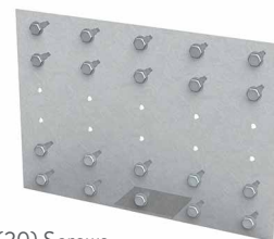
(20) Screws (12) at Header (8) at Jamb
