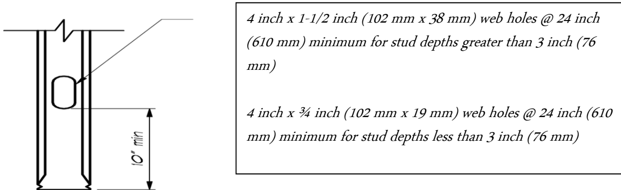
FIGURE 2—HOLE CONFIGURATION
