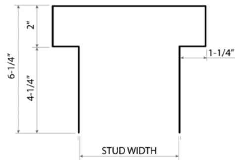
#8 2 HR, 4" total deflection
