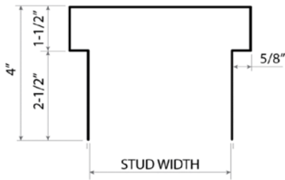
#3 1HR, 3" total deflection
