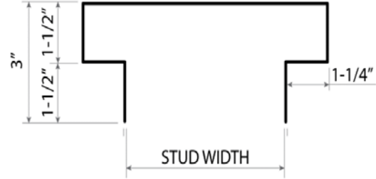
#6 2 HR, 2" total deflection
