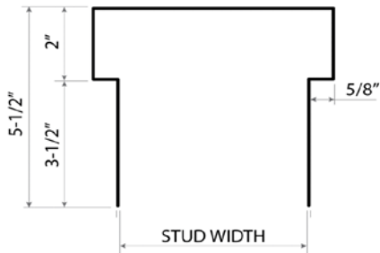
#3 1HR, 3" total deflection
