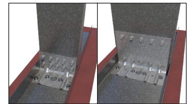
Figure 2 #12-24 screws
