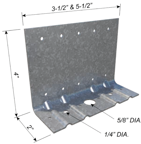
EasyClip T-Series Tall Anchor Clip
