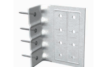
Location Options with (4) Anchors
