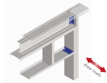
Head-to-Jamb Connections
