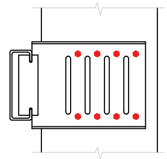
(8) #10 Screw Pattern Shown in a DRC6 Clip
