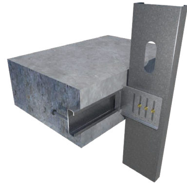
Drift Headed Rail (DHR) Installation
