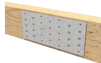
CDNP37 Installation
