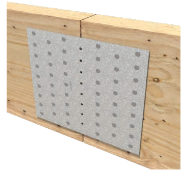
CDNP57 Installation
